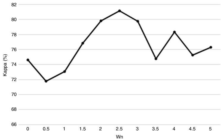
Fig. 5.7 Kappa values of the MonoLoop procedure
